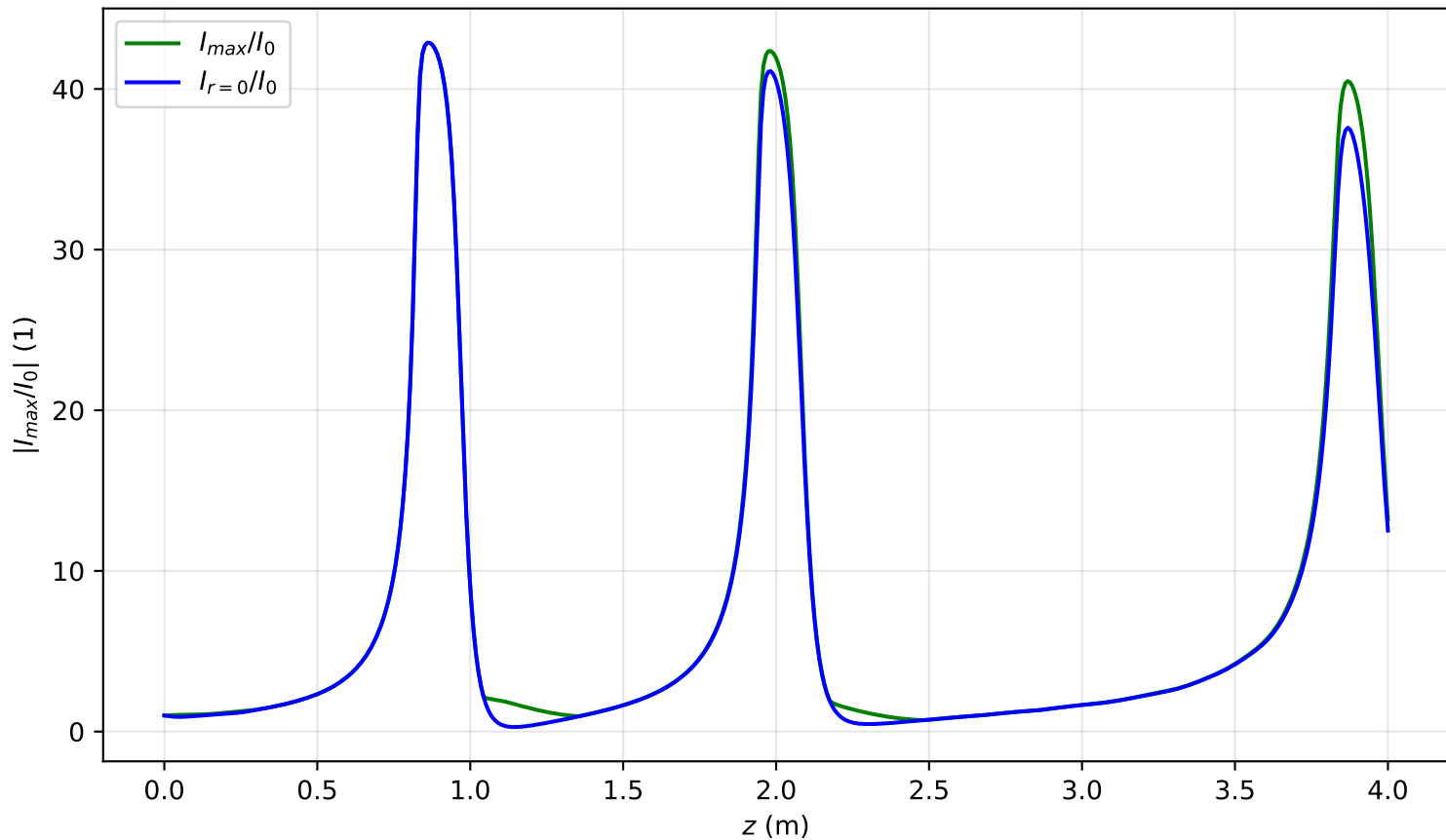
I_{max}(x = 0, y = 0, z)/I_0 , P_{in}=2.5P_{cr} , noisy input, artificial time
